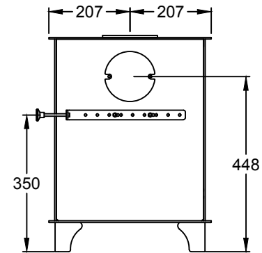
REAR ELEVATION DETAIL
