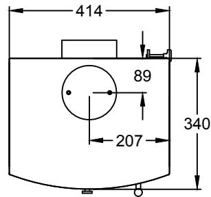
PLAN DETAIL
