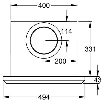
PLAN DETAIL
